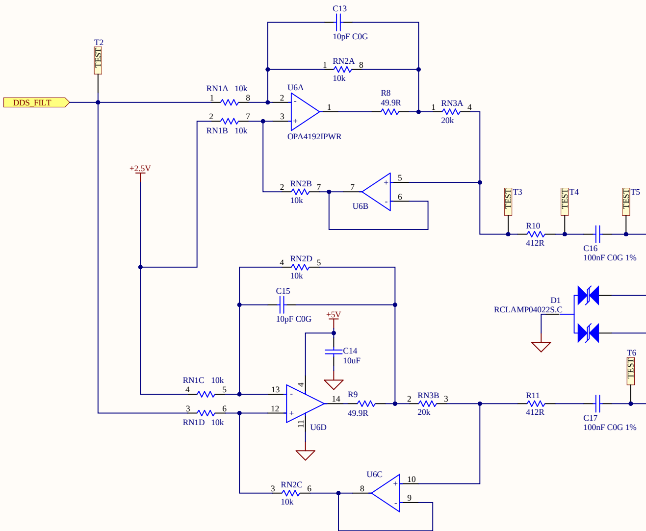
MIRRORED ENHANCED HOWLAND CURRENT PUMP
